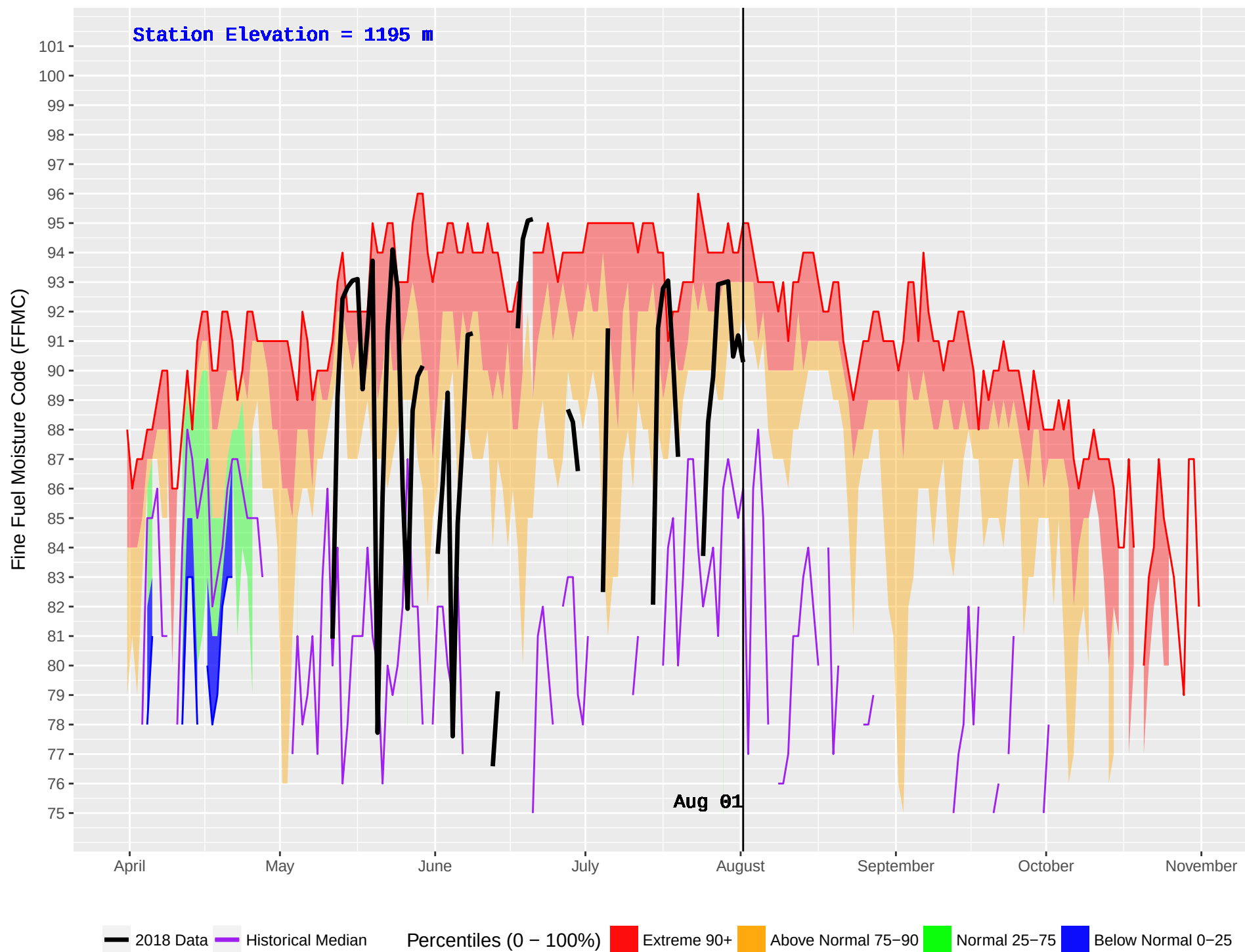
VALEMOUNT 2 (200) : Historical (1986–2016) and Current (2018) Daily Fine Fuel Moisture Code (FFMC)
